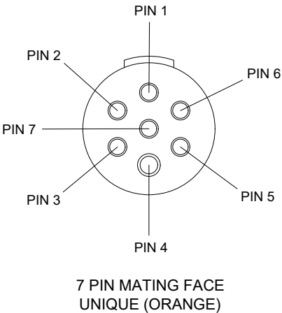
VIEW A
