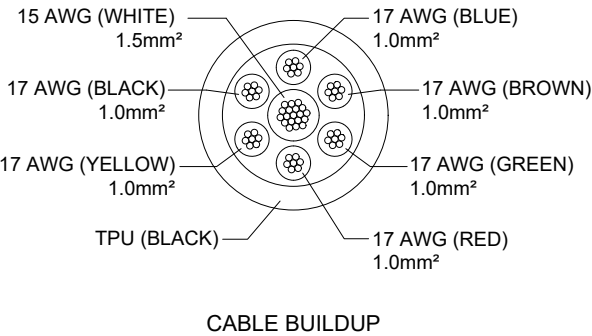
SECTION Z-Z
